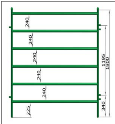
Round pipe's typical pitch
