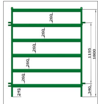
Square pipe's typical pitch
