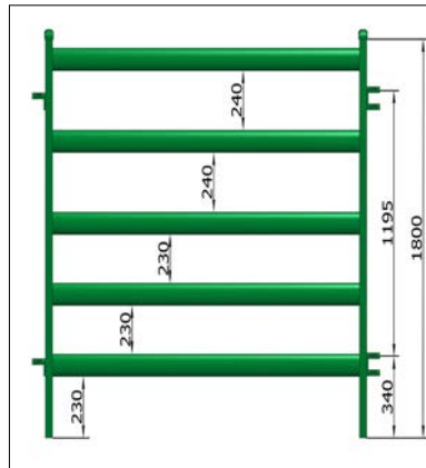
Oval pipe's typical pitch
